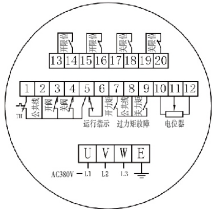
380V普通端子接线图 Wiring diagram of 380V common terminal
