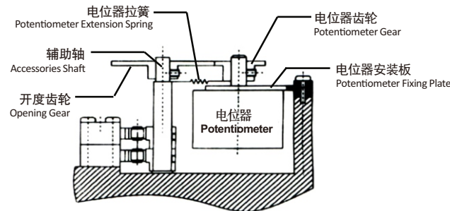
定位器的调整 Adjustment of potentiometer
