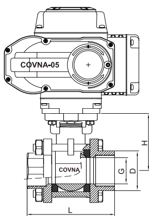
螺纹型 Threaded Type
