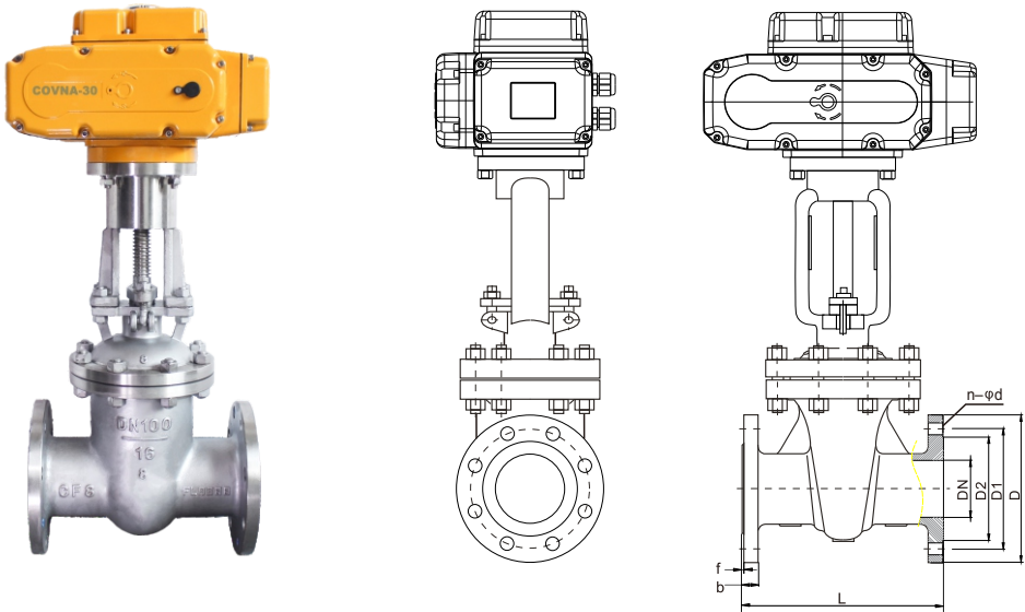
电动闸阀主要外形及连接尺寸(国标) Main Outline and Connecting ( MPa )
