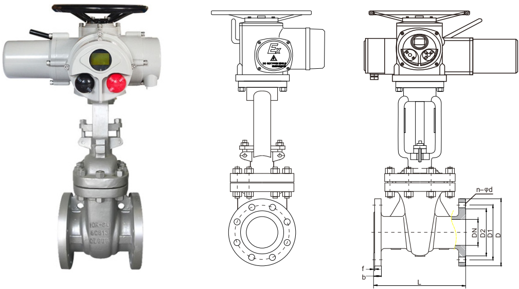
电动闸阀主要外形及连接尺寸(国标) Main Outline and Connecting ( GB )
