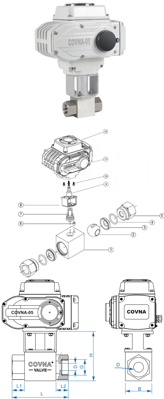
主要外形及连接尺寸 20MPa Main Outline and Connecting Flange Size
