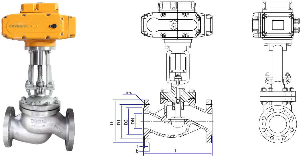
电动截止阀主要外形及连接尺寸(国标) Main Outline and Connecting ( MPa )
